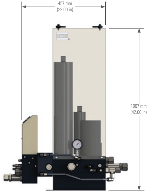
Model 293.22 Multi-Station Configuration Side View
