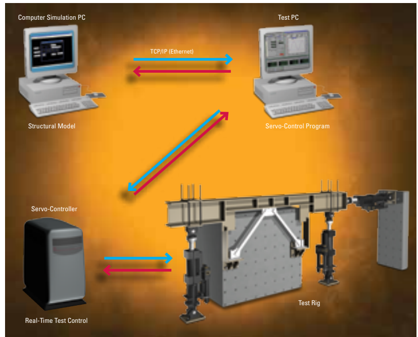
MTS Quasi-Static Hybrid Simulation
