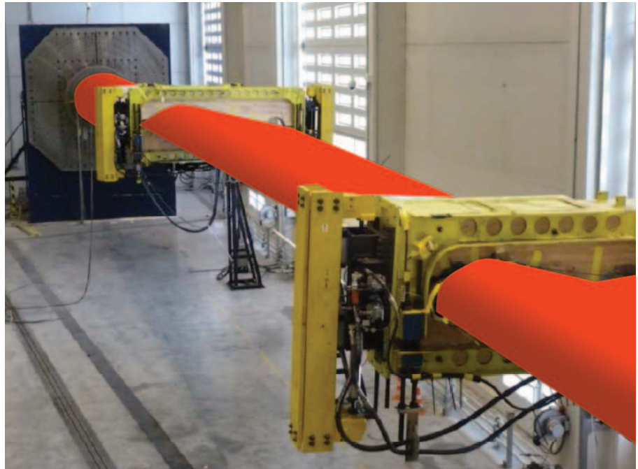
Inertial Resonance Excitation (IREX) Systems deployed for blade fatigue testing (blade visually obscured at customer's request)
