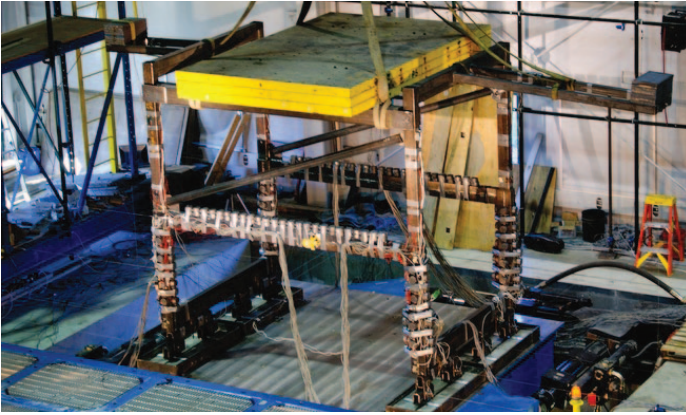
Large-scale, shake table test of container crane
